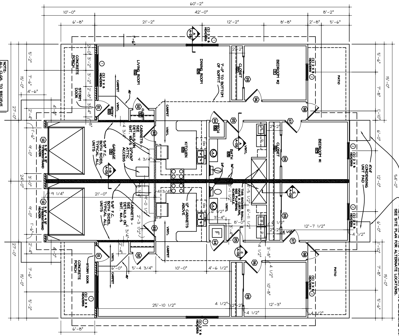
1 FLOOR PLAN SCALE 3/16" = 1'-0"
